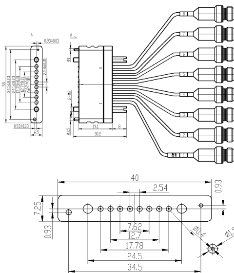
PCB Foot-Print Layout
